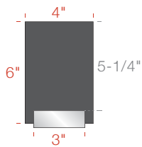
AS1L03-0604 3" w Bracket 3" h x 4" w Insert 5-1/4" h Display Area
