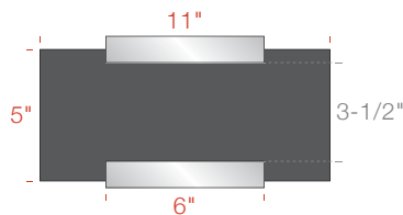
AS2L06-0511 AS2LB06-1111 (w/Backer) 6"w Bracket 5"h x 11"w Insert 3-1/2"h Display Area
