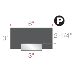
AS1L03-0306 3" w Bracket 3" h x 6" w Insert 2-1/4" h Display Area
