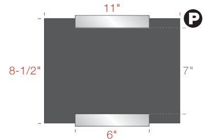
AS2L06-8511 AS2LB06-8511 (w/Backer) 6"w Bracket 8-1/2"h x 11"w Insert 7"h Display Area
