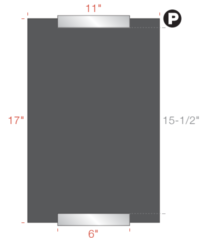
AS2L06-1711 AS2LB06-1711 (w/Backer) 6"w Bracket 17"h x 11"w Insert 15-1/2"h Display Area
