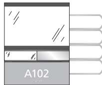
INFOEVWINSL-4R 10-11/16"h x 8-1/2"w (OD) 5-7/16"h x 8-1/2"w Display Insert 6-1/16"h x 8-1/2"w Window (OD) 1-1/2"h Slider 3" ADA Insert
