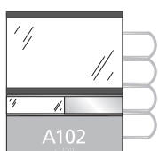
INFO2EVWINSL-4R 10-11/16"h x 8-1/2"w (OD) 5-7/16"h x 8-1/2"w Display Insert 6-1/16"h x 8-1/2"w Window (OD) 1-1/2"h Slider 3" ADA Insert
