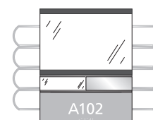
INFO2EVWINSL-4RL 10-11/16"h x 8-1/2"w (OD) 5-7/16"h x 8-1/2"w Display Insert 6-1/16"h x 8-1/2"w Window (OD) 1-1/2"h Slider 3" ADA Insert
