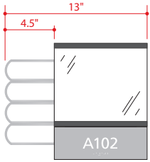
INFOEVWIN-4L 10-11/16"h x 8-1/2"w (OD) 7"h x 8-1/2"w Display Insert 7-5/8"h x 8-1/2"w Window (OD) 3" ADA Insert
