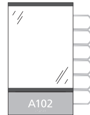
INFO2EVWIN-6R 14-11/16"h x 8-1/2"w (OD) 11"h x 8-1/2"w Display Insert 11-5/8"h x 8-1/2"w Window (OD) 3" ADA Insert
