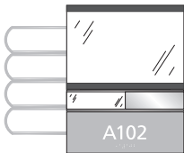
INFOEVWINSL-4L 10-11/16"h x 8-1/2"w (OD) 5-7/16"h x 8-1/2"w Display Insert 6-1/16"h x 8-1/2"w Window (OD) 1-1/2"h Slider 3" ADA Insert
