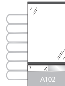
INFOEVWINSL-8L 17-11/16"h x 8-1/2"w (OD) 12-7/16"h x 8-1/2"w Display Insert 13-1/16"h x 8-1/2"w Window (OD) 1-1/2" Slider 3" ADA Insert
