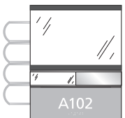
INFO2EVWINSL-4L 10-11/16"h x 8-1/2"w (OD) 5-7/16"h x 8-1/2"w Display Insert 6-1/16"h x 8-1/2"w Window (OD) 1-1/2"h Slider 3" ADA Insert
