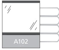
INFOEVWIN-4R 10.68"h x 7.5"w (OD)* 7"h x 8-1/2"w Display Insert 7-5/8"h x 7-1/2"w Window (OD)* 3"h ADA Insert
