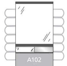
INFO2EVWINSL-6RL 14-11/16"h x 8-1/2"w (OD) 9-7/16"h x 8-1/2"w Display Insert 10-1/16"h x 8-1/2"w Window (OD) 1-1/2" Slider 3" ADA Insert
