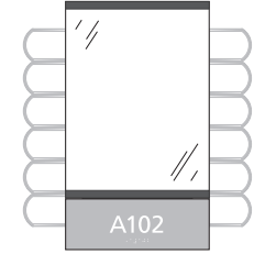
INFO2EVWIN-6RL 14-11/16"h x 8-1/2"w (OD) 11"h x 8-1/2"w Display Insert 11-5/8"h x 8-1/2"w Window (OD) 3" ADA Insert
