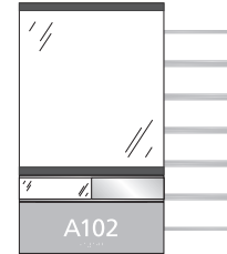
INFOEVWINSL-6R 14-11/16"h x 8-1/2"w (OD) 9-7/16"h x 8-1/2"w Display Insert 10-1/16"h x 8-1/2"w Window (OD) 1-1/2" Slider 3" ADA Insert
