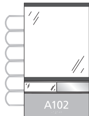
INFO2EVWINSL-6L 14-11/16"h x 8-1/2"w (OD) 9-7/16"h x 8-1/2"w Display Insert 10-1/16"h x 8-1/2"w Window (OD) 1-1/2" Slider 3" ADA Insert
