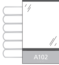
INFOEVWIN-6L 14-11/16"h x 8-1/2"w (OD) 11"h x 8-1/2"w Display Insert 11-5/8"h x 8-1/2"w Window (OD) 3" ADA Insert
