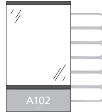
INFOEVWIN-6R 14-11/16"h x 8-1/2"w (OD) 11"h x 8-1/2"w Display Insert 11-5/8"h x 8-1/2"w Window (OD) 3" ADA Insert
