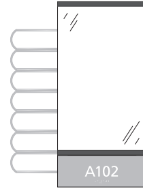
INFOEVWIN-8L 17-11/16"h x 8-1/2"w (OD) 14"h x 8-1/2"w Display Insert 14-5/8"h x 8-1/2"w Window (OD) 3" ADA Insert
