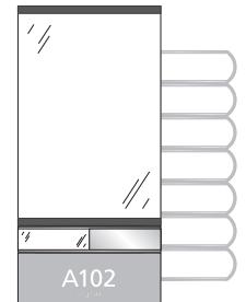
INFOEVWINSL-8R 17-11/16"h x 8-1/2"w (OD) 12-7/16"h x 8-1/2"w Display Insert 13-1/16"h x 8-1/2"w Window (OD) 1-1/2" Slider 3" ADA Insert
