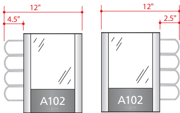
INFO2AR01-4L (Left) 10.08"h x 7.5"w (OD) 7"h x 6"w - Display Area 3"h - ADA Band
