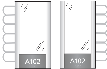
INFO2AR01-6L (Left) 14.08"h x 7.5"w (OD) 11"h x 6"w - Display Area 3"h - ADA Band
